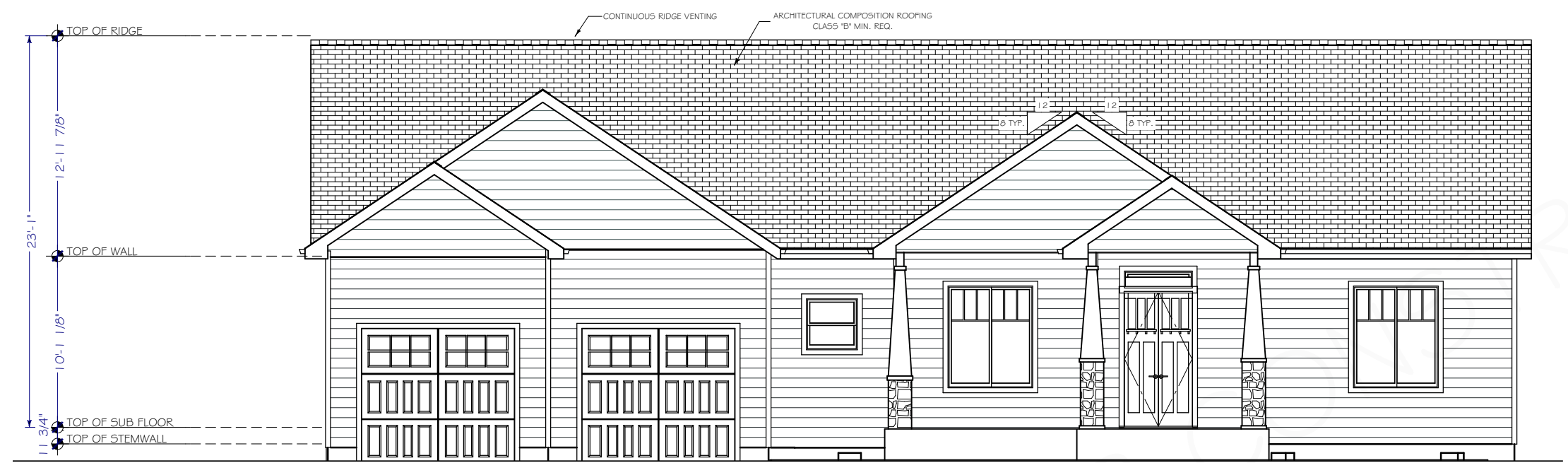
FRONT ELEVATION 1/8 in = 1 ft
